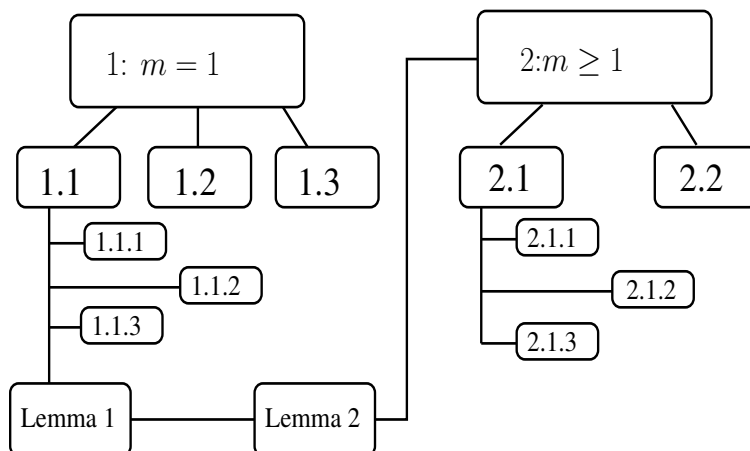
Figure 2: Logical flow of the proof.
