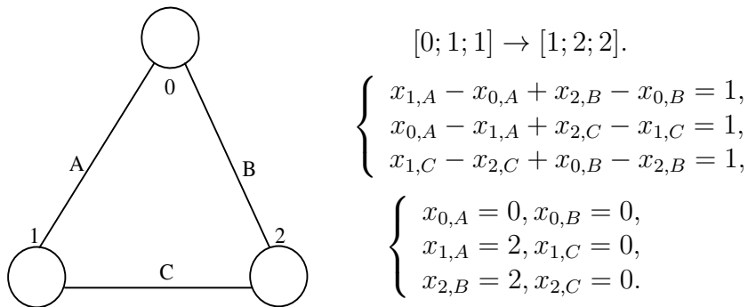
Figure 1: (a). The counterexample G ( p=3 ) (b). The system and its solution
