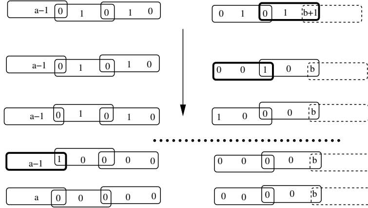
Figure 4: Backward restoration. Each pictured "step" applies Observation 1 on one edge, starting from e_{k-1} down to e_1 . On each row the the scheduled edge is darkened. For simplicity we pictured the particular situation when no two hyperedges intersect at a set of cardinality larger than one, hence all hyperedges have "internal" nodes (whose state is 1 after the forward moves). The scheduled nodes are these internal nodes. Last row represents the resulting state.
