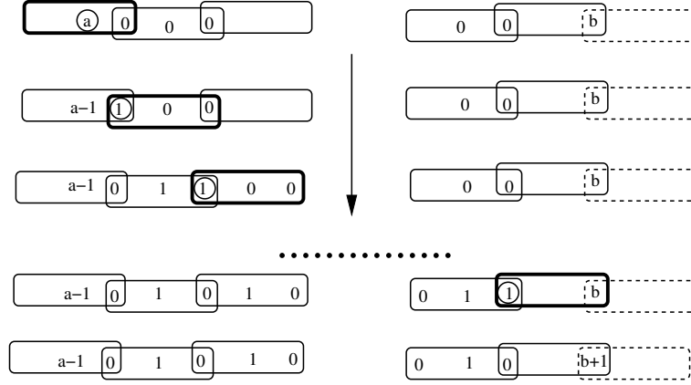
Figure 3: Forward propagation of nonzero values. Initially node v_1 has value a and target node v_k has value b (with edge e_k being dashed). On each row the node scheduled at that stage is circled, with the scheduled edge being darkened. Scheduling a node has the effect of decreasing its label by one (mod p ) and increasing the label of all other nodes in the edge by one (mod p ). For simplicity we pictured the situation when no two hyperedges intersect at a set of cardinality larger than one. Thus no label 2 is created and all hyperedges have “internal” nodes (whose new state is 1). Last row represents the resulting state.
